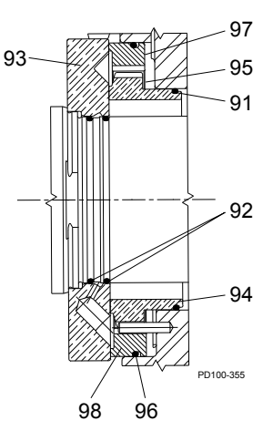
Aseptic Design Double Mechanical Seal (213, 323 U2 ONLY)
