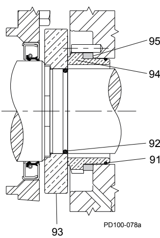
Standard Single Mechanical Seal
