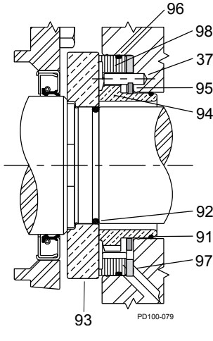
Standard Double Mechanical Seal
