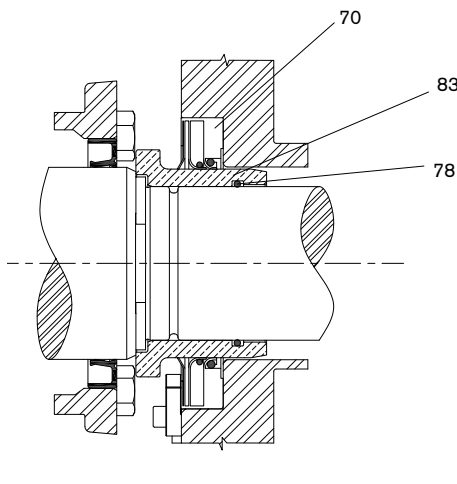
Triple Lip Seal
