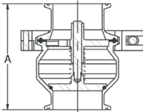
O-ring seat with light spring for low flow resistance.
