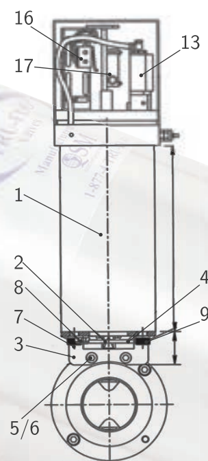
K1111-2 Solenoid & Mechanical Limit Switch
