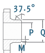
83-20 Socket Weld End
