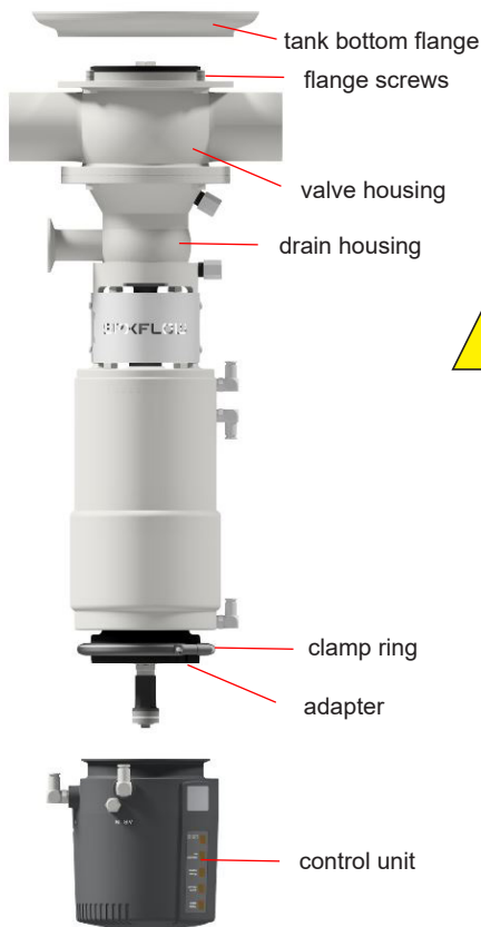
fig. 12.1. DP4 SL valve
