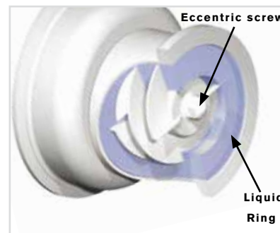
Eccentric screw forms liquid ring
