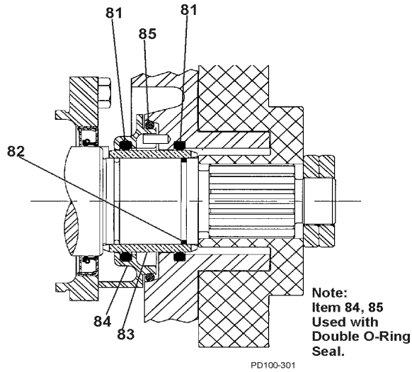
O-Ring Seal
