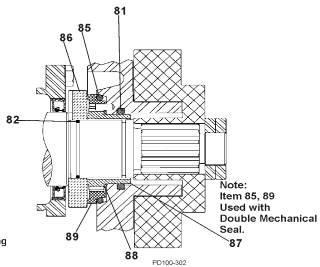
Mechanical Seal
