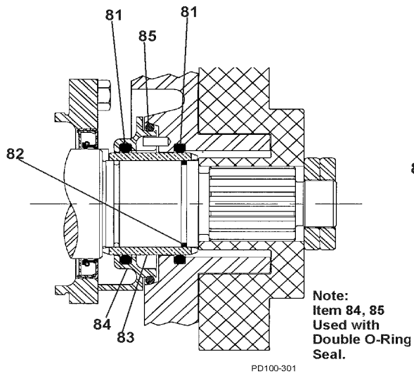
O-Ring Seal
