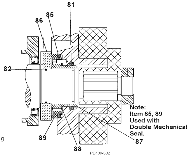
Mechanical Seal
