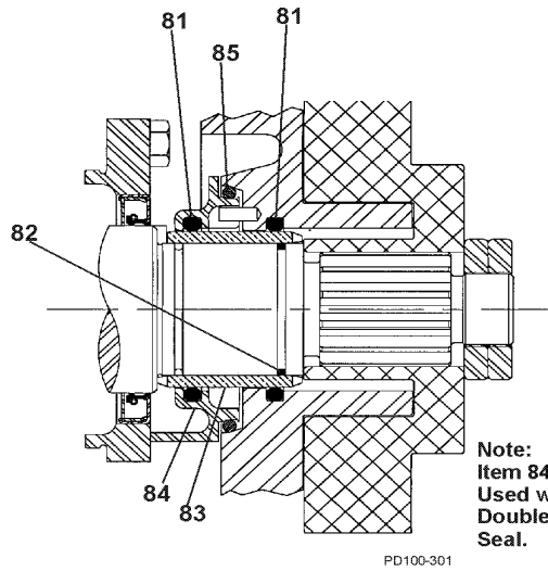
O-Ring Seal
