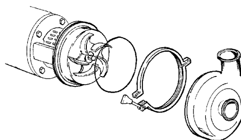
Figure 54 - Remove Casing Clamp, Casing and O-ring
