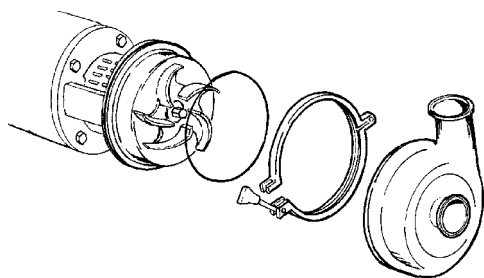
Figure 46 - Install Casing
