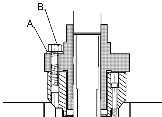
Figure 55 - Removal of Wet End
