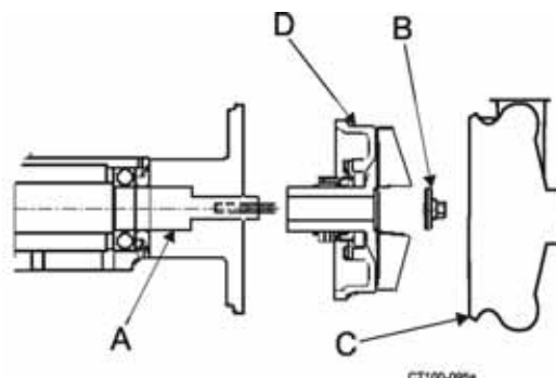
Figure 61 - Installing Impeller Assembly item B).
