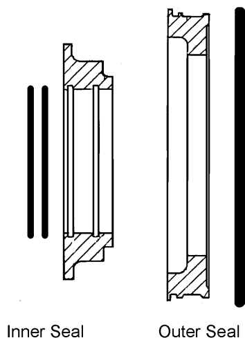
Figure 52 - Seal Configuration
