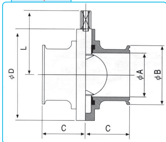
Tri-clamp Ends
