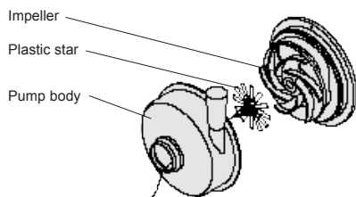
Fig. 8: Place plastic star against impeller
